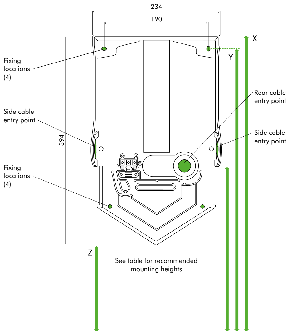
REAR ELEVATION
